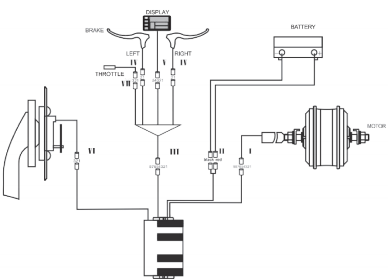
Electric Circuit Diagram
