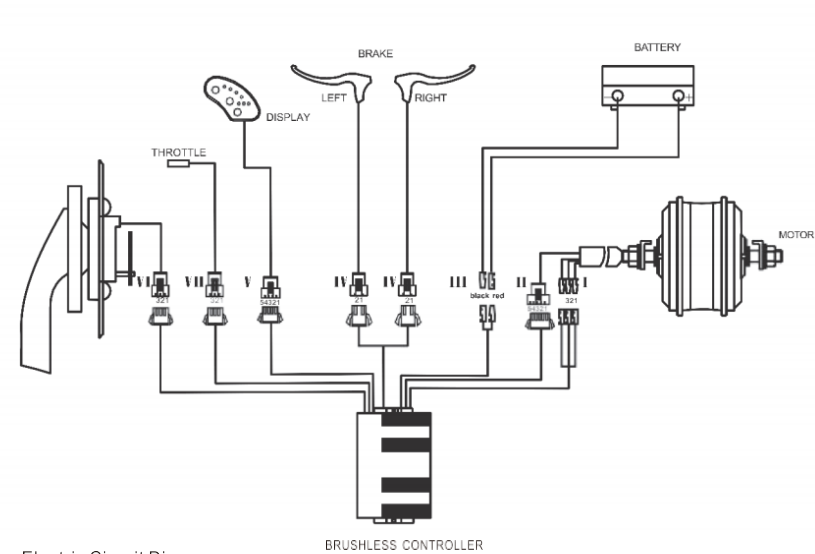
Electric Circuit Diagram
